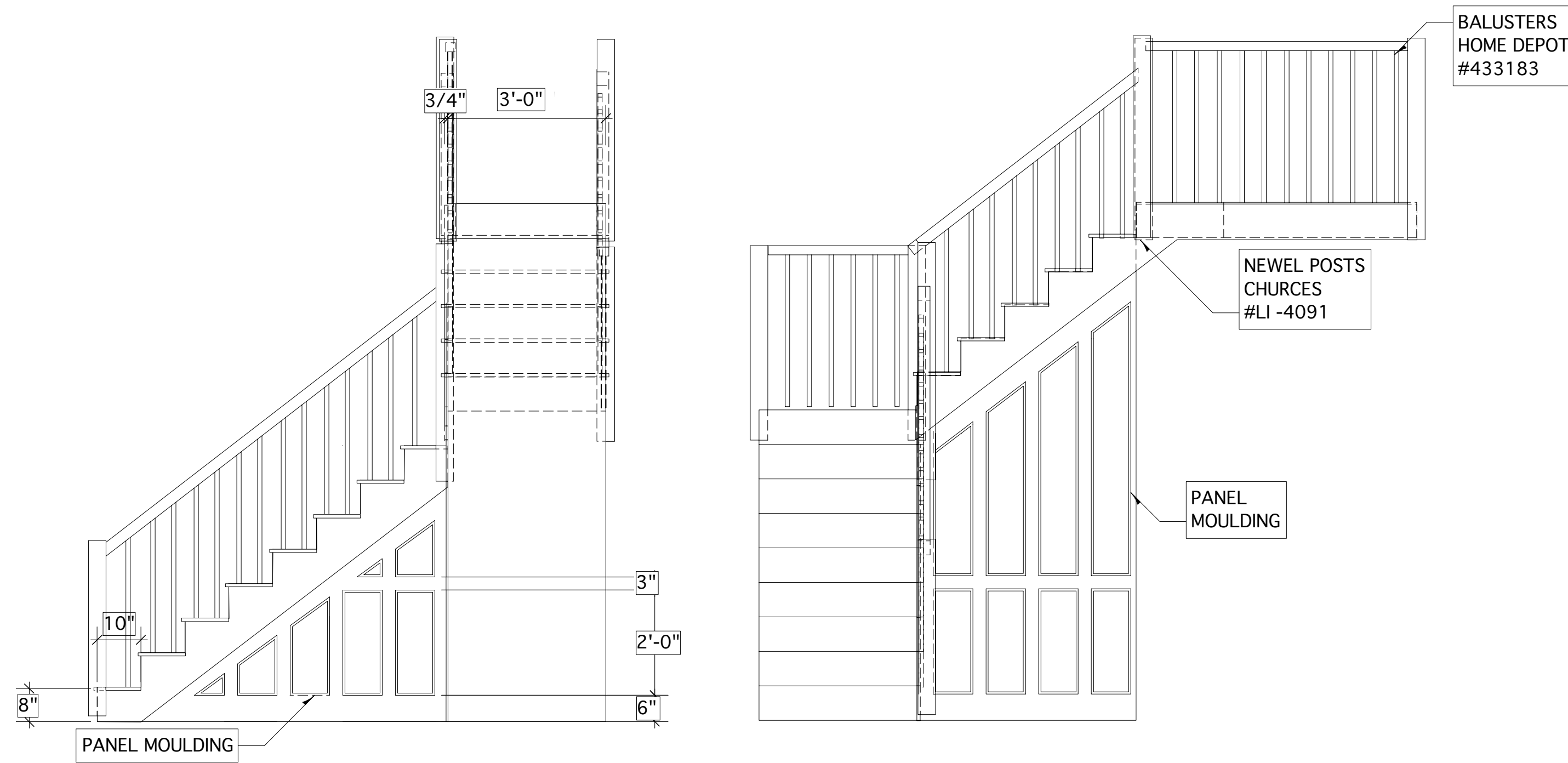
STAIRCASE ELEVATION
