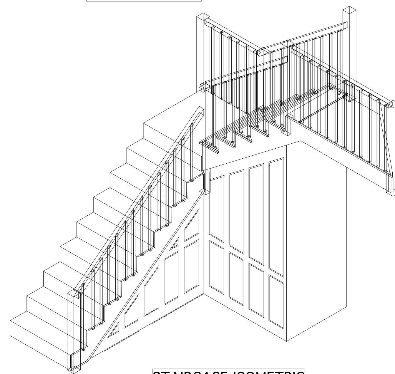
STAIRCASE ISOMETRIC
